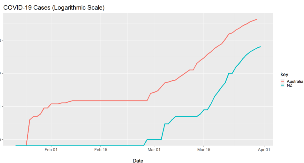
Figure 7: COVID-19 Cases (Logarithmic scale) in New Zealand & Australia
