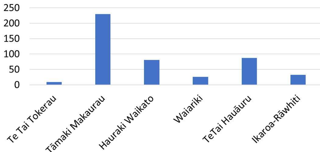
Figure 1: COVID-19 Cases based on WOCA region
