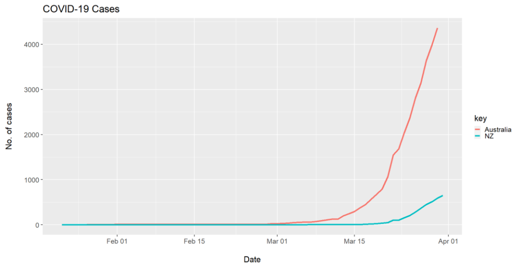
Figure 6: COVID-19 Cases in New Zealand & Australia
